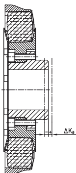
Axial displacement
