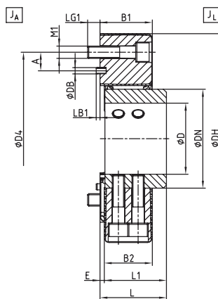
Size 360 - 560
