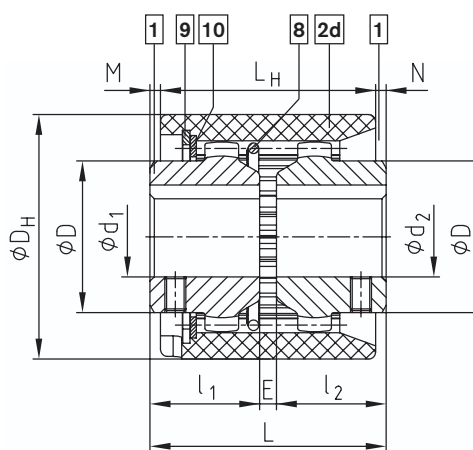
Type Spec.-I
