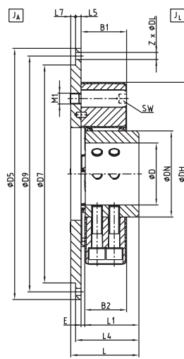
Size 360
