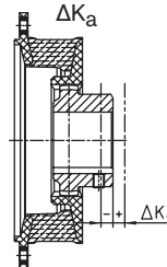
Axial displacement \Delta K_a
