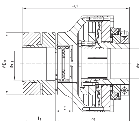
Hub type 6.0
