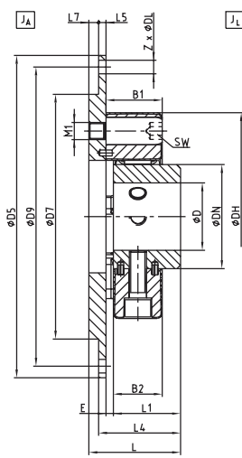
Size 12 - 280
