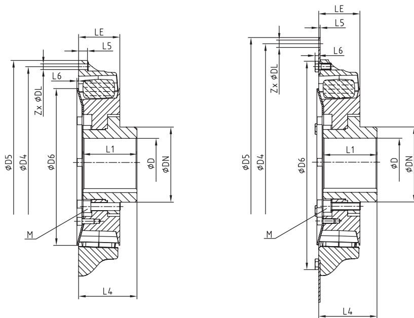
Type A (direct flange connection)
