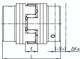
Axial displacement \Delta K_a
