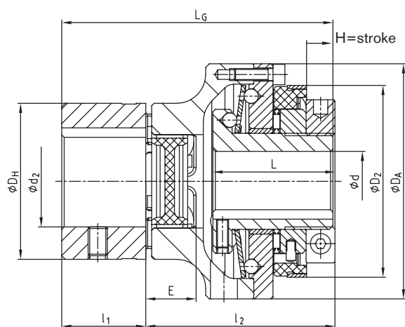
Hub type 1.0
