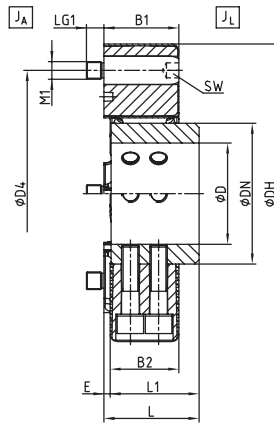
Size 360
