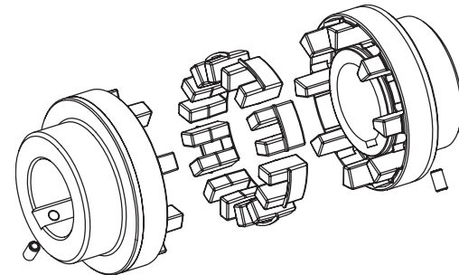
Size 140 - 280
