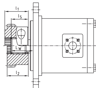
Clamping hub
