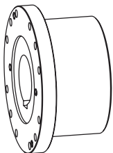
Type 1.0 hub with feather keyway and setscrew
