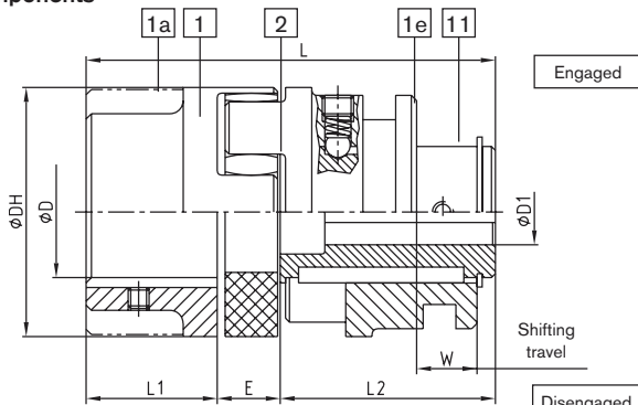
Type SD
