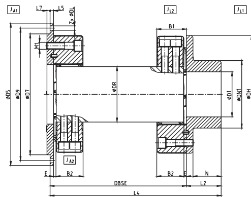
Size 360 - 560
