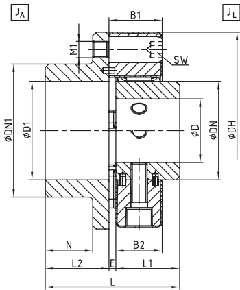
Size 12 - 280
