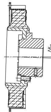
Angular displacement
