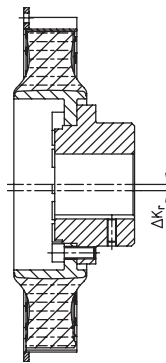
Radial displacement
