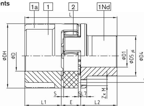
Type FNN
