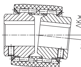
Angular displacement
