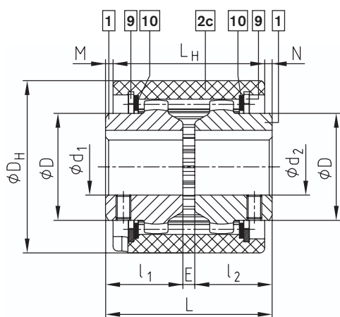
Type AS
