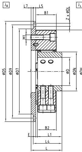
Size 360 - 560
