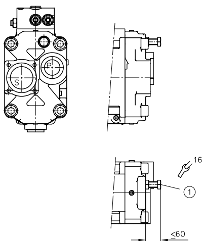
1 Stroke limitation ( V_g approx. 5 \text{ cm}^3/\text{rev.} )
