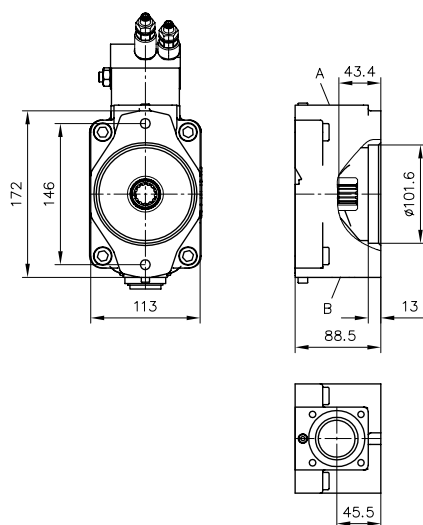
Coding C 014 (SAE-B 2-hole)
