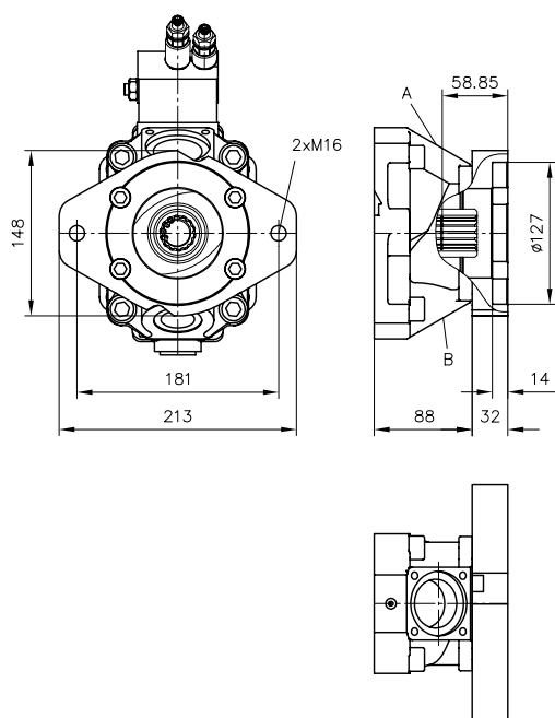
Coding C 027 (SAE-C 2-hole)
