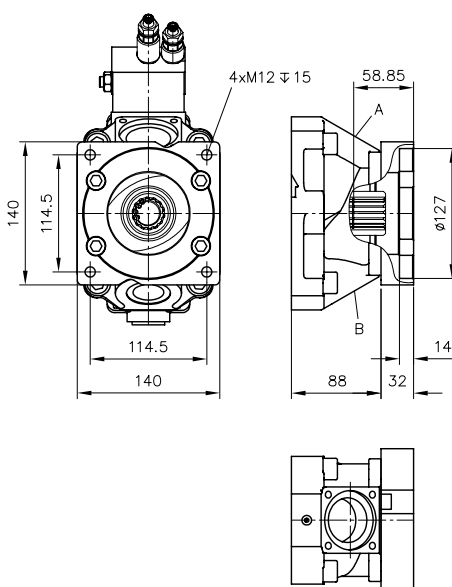
Coding C 028 (SAE-C 4-hole)
