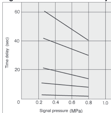
Signal Pressure vs. Time Delay
