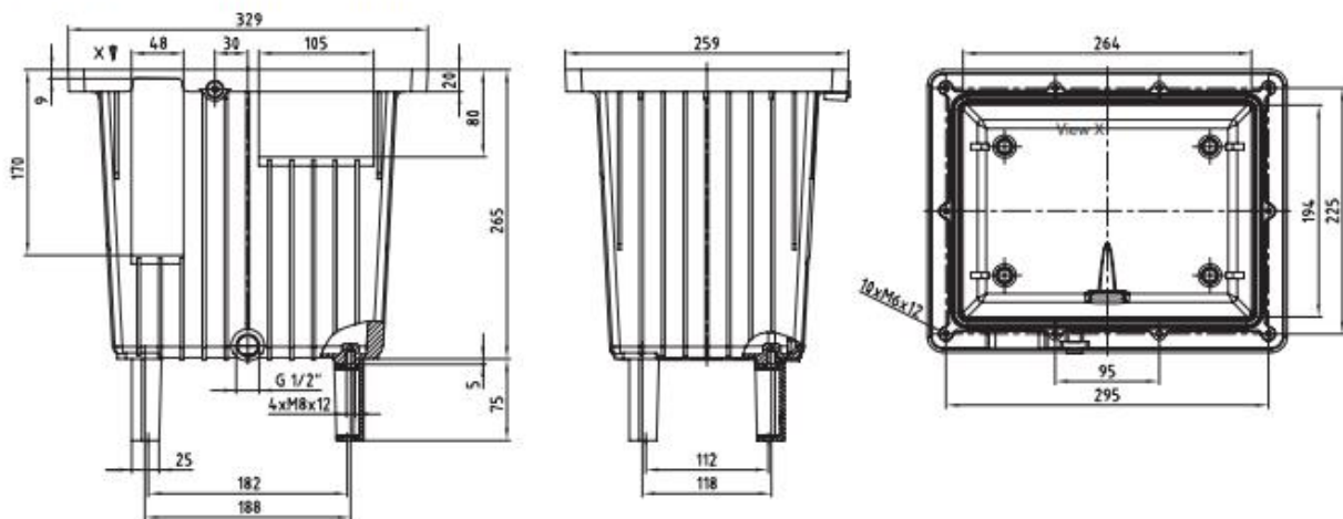
Tank with oil collecting groove BAK 13
