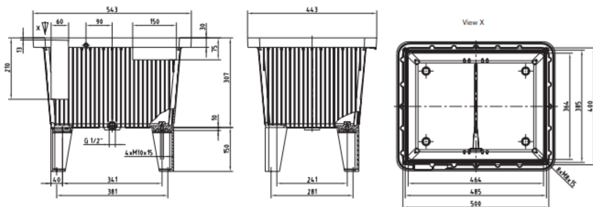
Tank with oil collecting groove BAK 44
