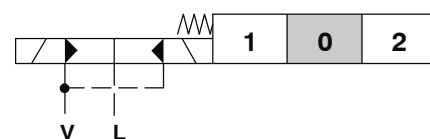
Scheme ISO 1219
