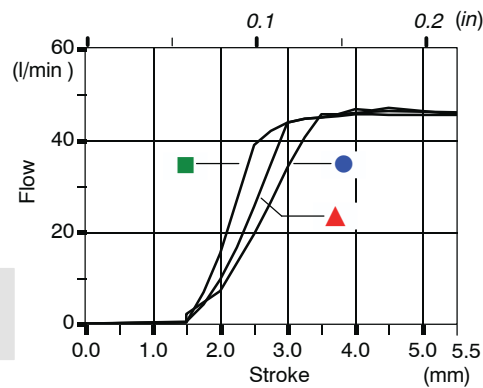
Spool metering A→T
