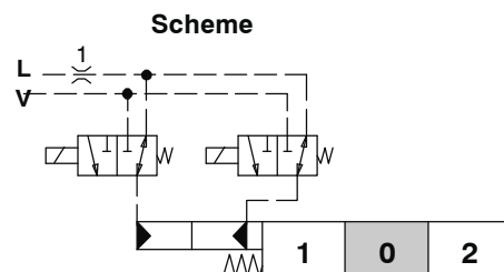
Scheme ISO 1219
