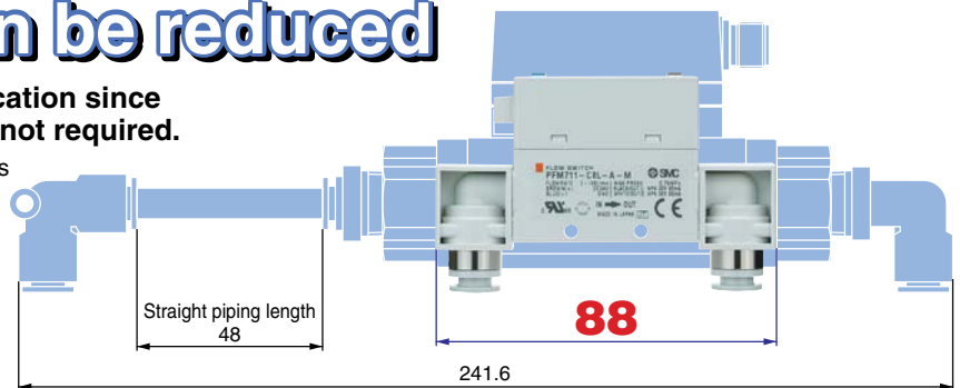
Comparison with the conventional model PF2A711 (10 to 100 ℓ/min) when ø6 one-touch fittings are attached.
