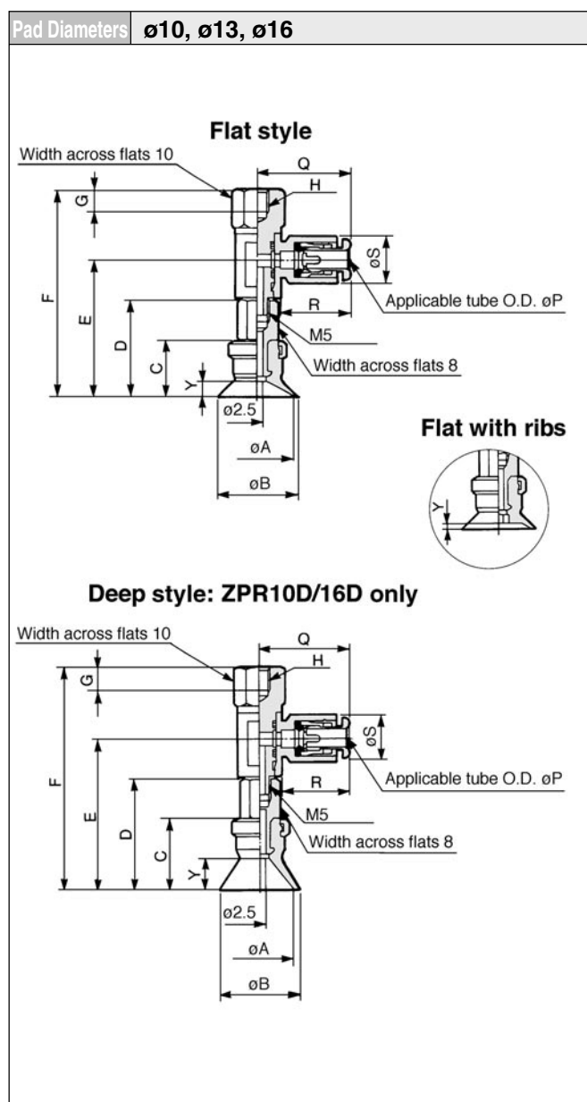
Flat style/Flat with ribs
