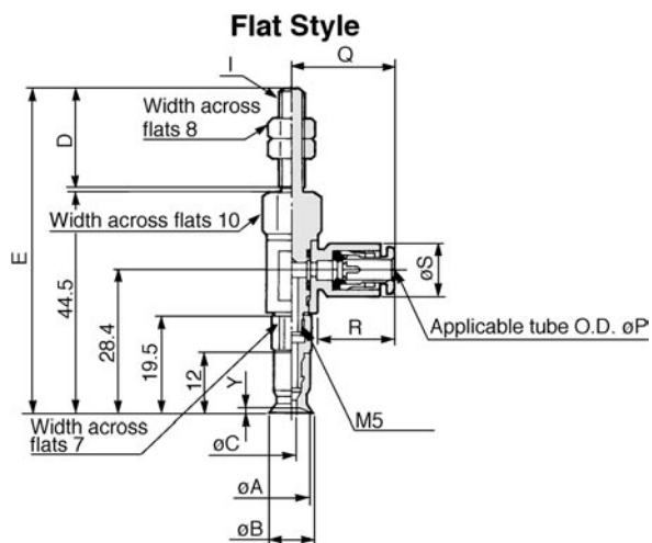
Pad Diameters ø2, ø4 ,ø6, ø8
