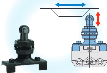
Roller plunger
