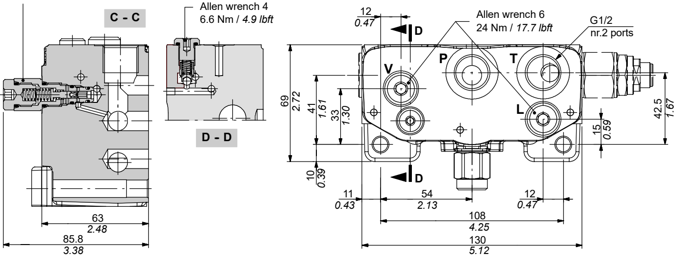
Pressure reducing valve VRPF Wrench 19 - 42 Nm / 31 lbft
