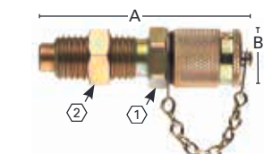
Bulkhead Couplings
