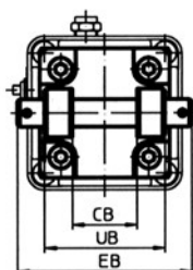
Double Clevis Type
