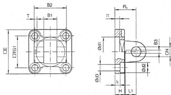
Rear Single Clevis CS
