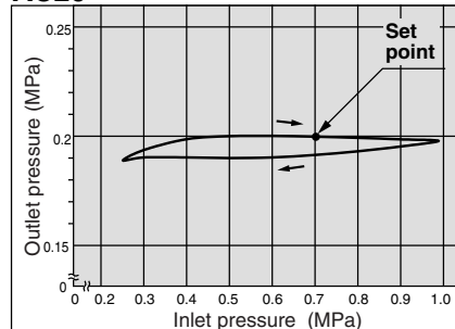
AC40
