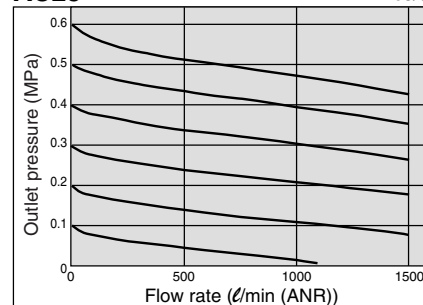
AC40-06 Rc3/4
