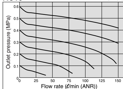
AC30 Rc3/8
