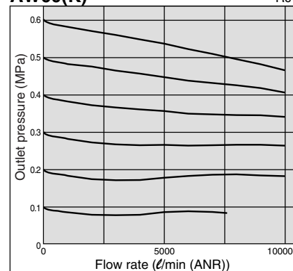
AW60(K) Rc1
