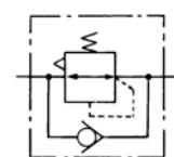
Regulator with Backflow Function
