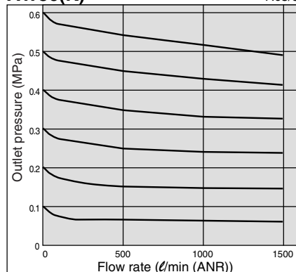
AW30(K) Rc3/8
