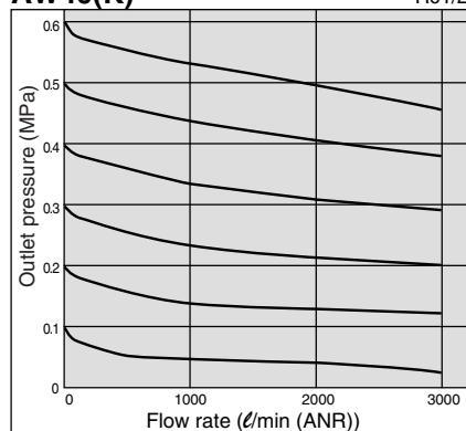
AW40(K) Rc1/2
