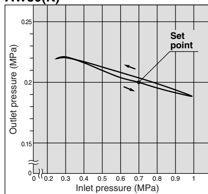
AW30(K)
