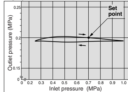
AC40-06
