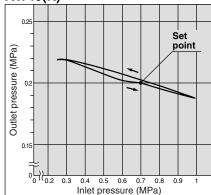
AW40(K)
