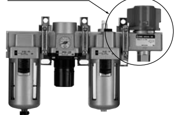
3-port valve for residual pressure release
