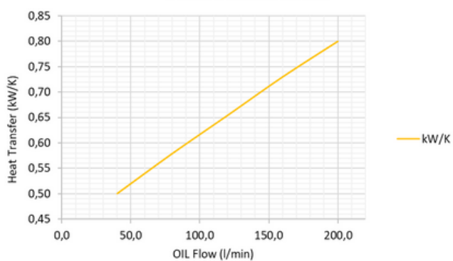
Performance Curve
