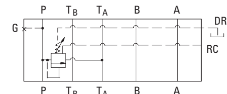
DGMC-5-PT-**-E-RC-**-30
