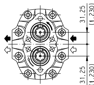
Flange T2
