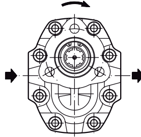
CLOCKWISE ROTATION
