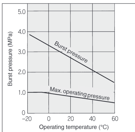
Burst Pressure Characteristics Curve
