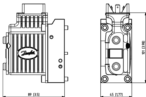
Dimensions drawing
