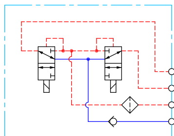
PVEO-HP Schematic
