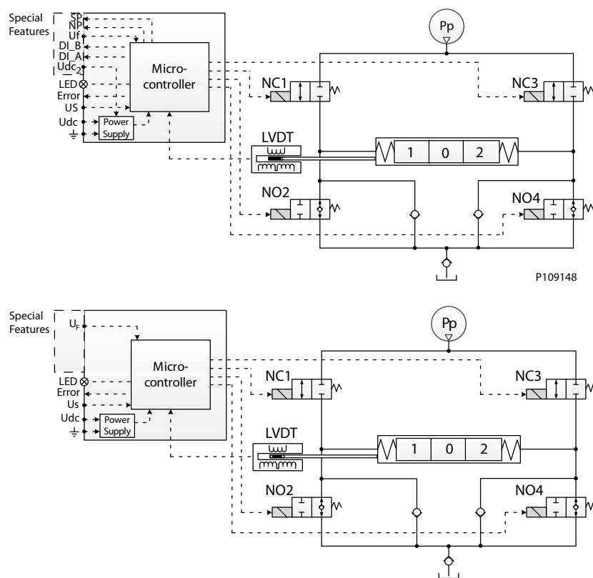
PVEH-FLA functionality diagram
